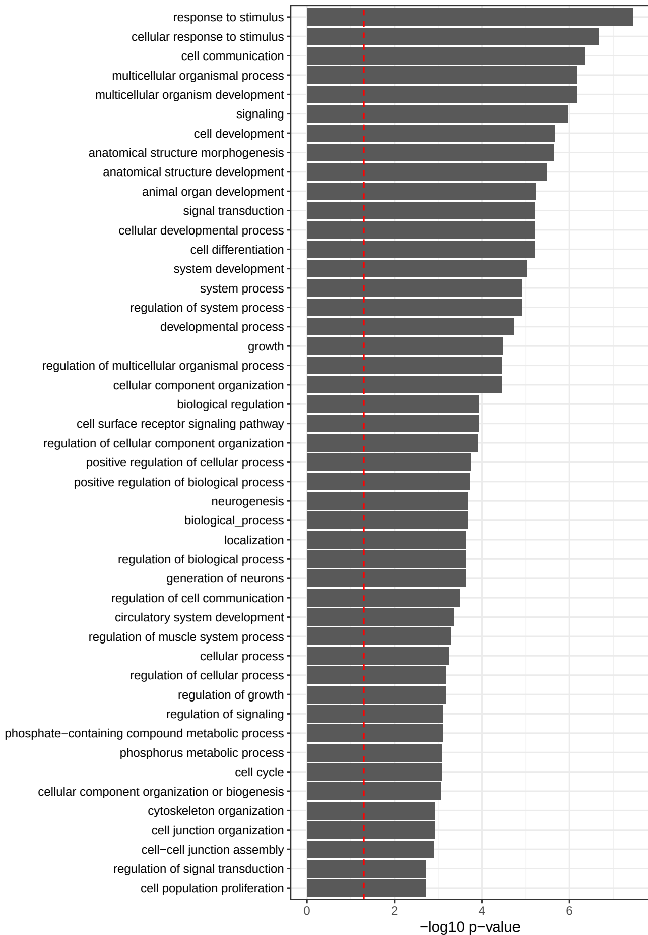
24 hour down DNR_DAR_DEG pairs (within 20
